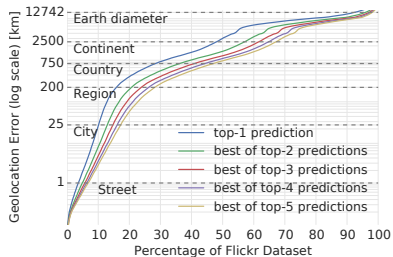
Fig. 3. Geolocation accuracy of the top- k most confident predictions on 2.3M Flickr photos. (Lower right is best)
