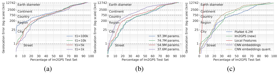
Fig. 9. (a) Performance for different resolutions of S2 discretization representing different trade-offs between the number of classes and the number of training images per class (Tab. 1b). (b) Performance for different numbers of model parameters. The full model has 97.3M parameters. (c) Comparison of PlaNet with image retrieval based on local features and CNN embeddings
