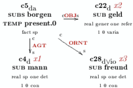
Figure 2: HaGenLex entry showing an example sentence for the German verb “borgen.1.1” (“to borrow”). The sentence is literally “The man borrows himself money from the friend.”
