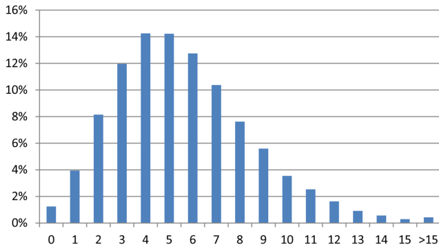
Figure 3: The distribution of the number of topic annotations per snippet, over AMBIENT and ODP-239. Column 0 corresponds to the percentage of snippets that did not get annotated by TAGME.
