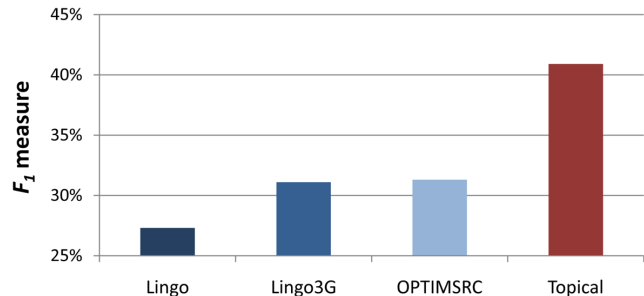
Figure 4: Evaluation of different SRC systems over the ODP-239 dataset.
