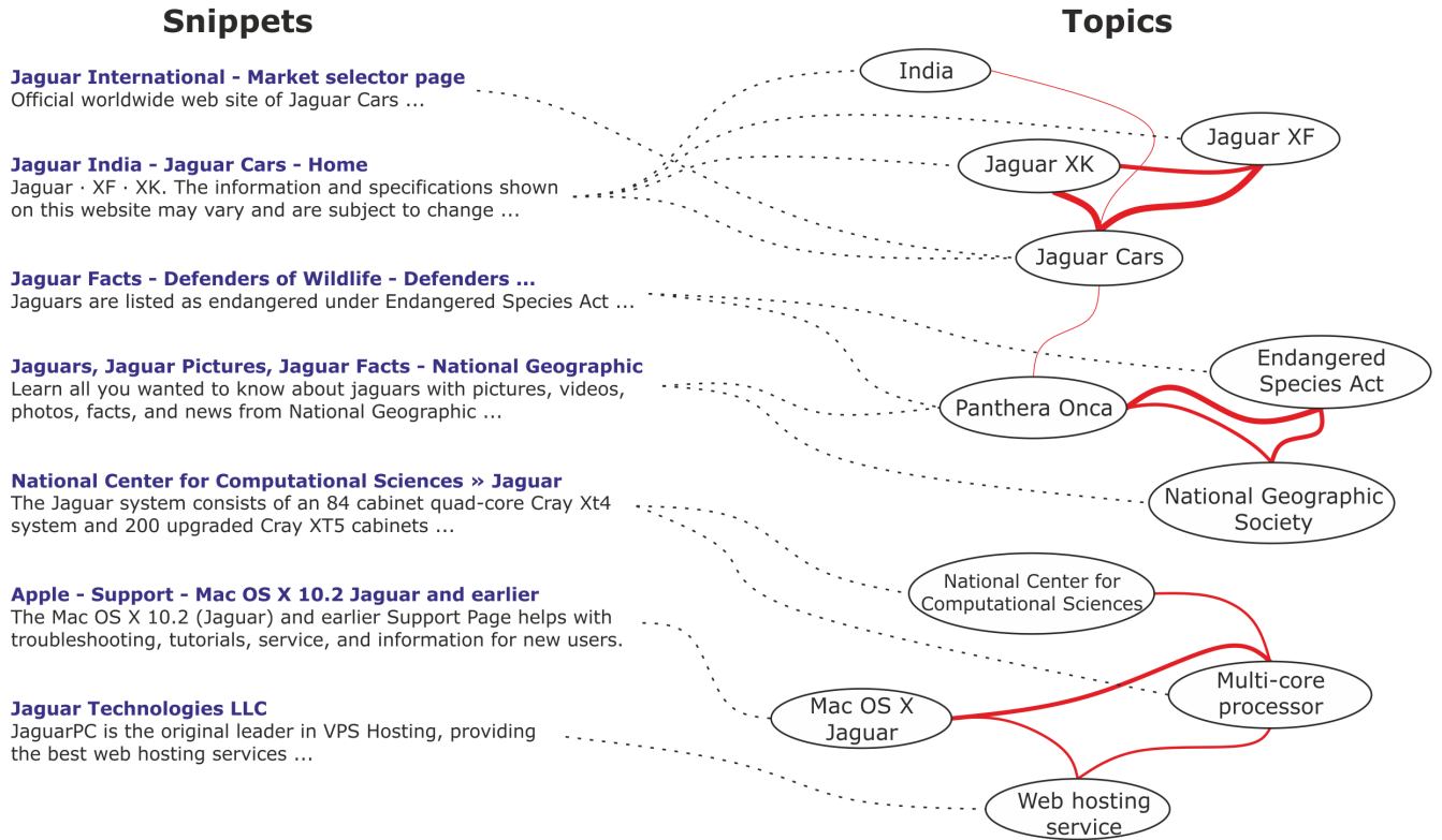
Figure 2: The graph of topics representation for texts.
