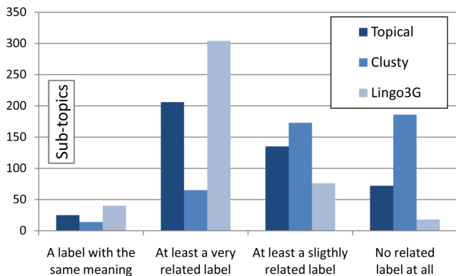
Figure 6: Evaluation of the effectiveness of the cluster labeling produced for all queries of the TREC-100 dataset by our tested systems.
