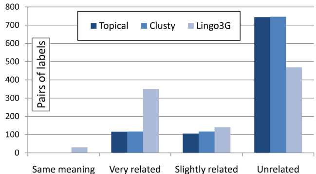
Figure 5: Evaluation of diversification of labeling produced for all queries of the TREC-100 dataset by our tested systems.
