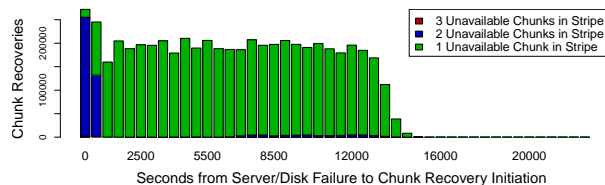
Figure 9: Example chunk recovery after failure bursts.
